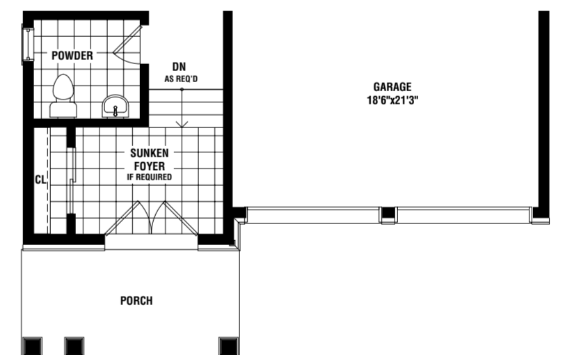
FIRST FLOOR ELEV. 'B'
