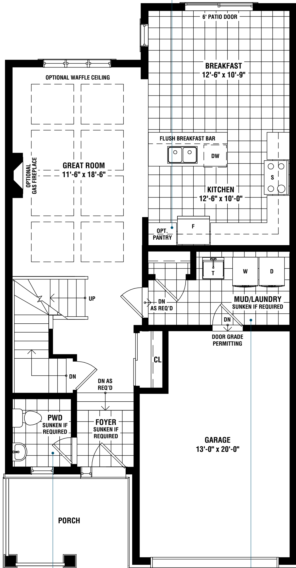
1ST FLOOR ELEVATION A
