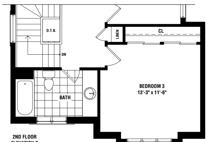
2ND FLOOR ELEVATION B
