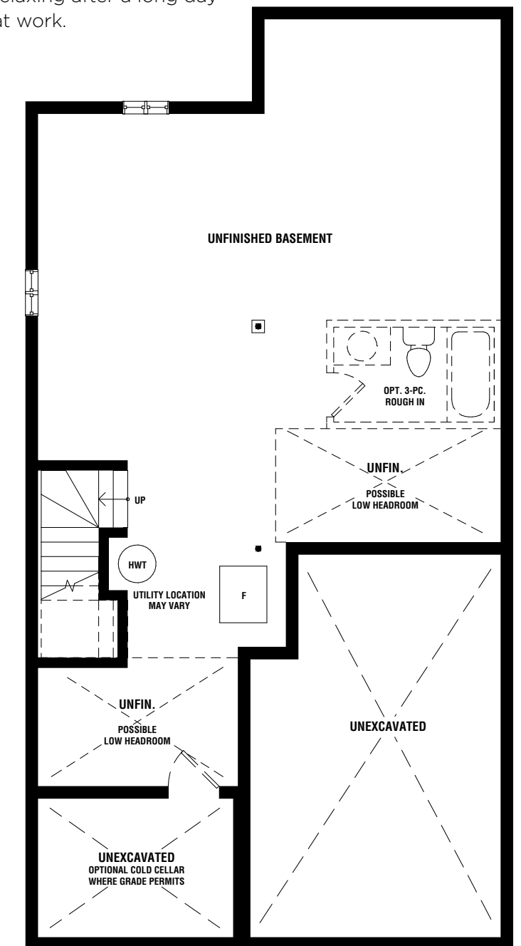
BASEMENT
